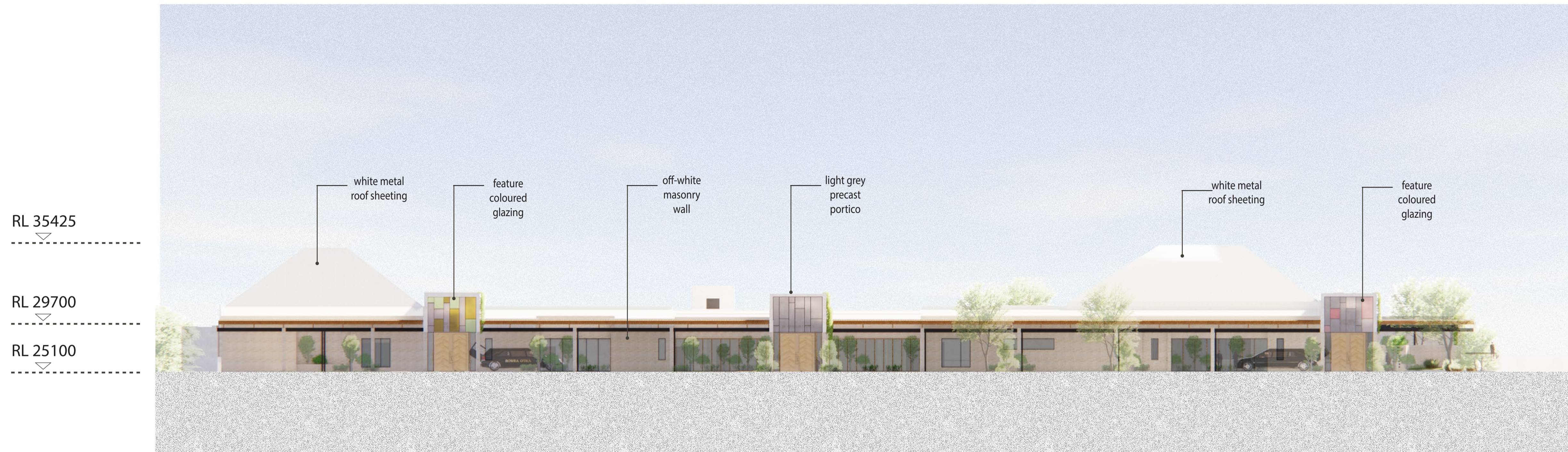
Elevation North
