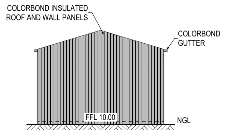
SOUTH ELEVATION (1:75) (NORTH ELEVATION SIMILAR)
