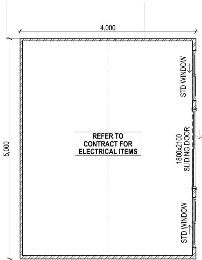
FLOOR PLAN (1:50)
