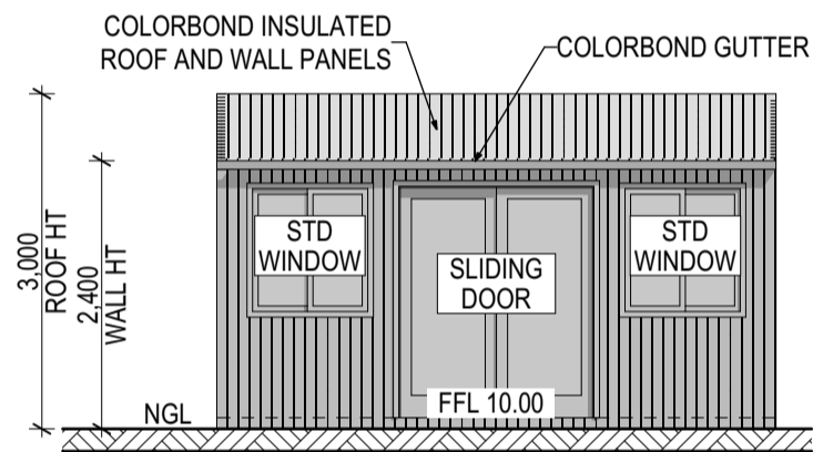
EAST ELEVATION (1:75)
