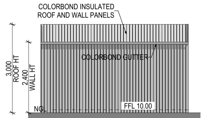
WEST ELEVATION (1:75)
