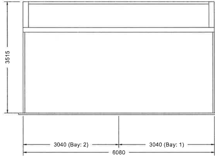
LEFT ELEVATION
