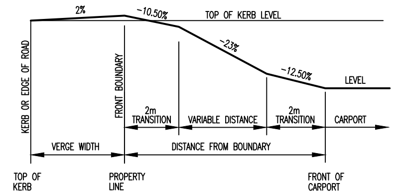
TYPICAL PROFILE OF TREATMENT BELOW KERB
