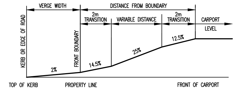
TYPICAL PROFILE OF TREATMENT ABOVE KERB
