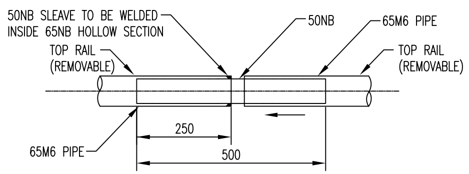
DETAIL 2 (NOT TO SCALE)
