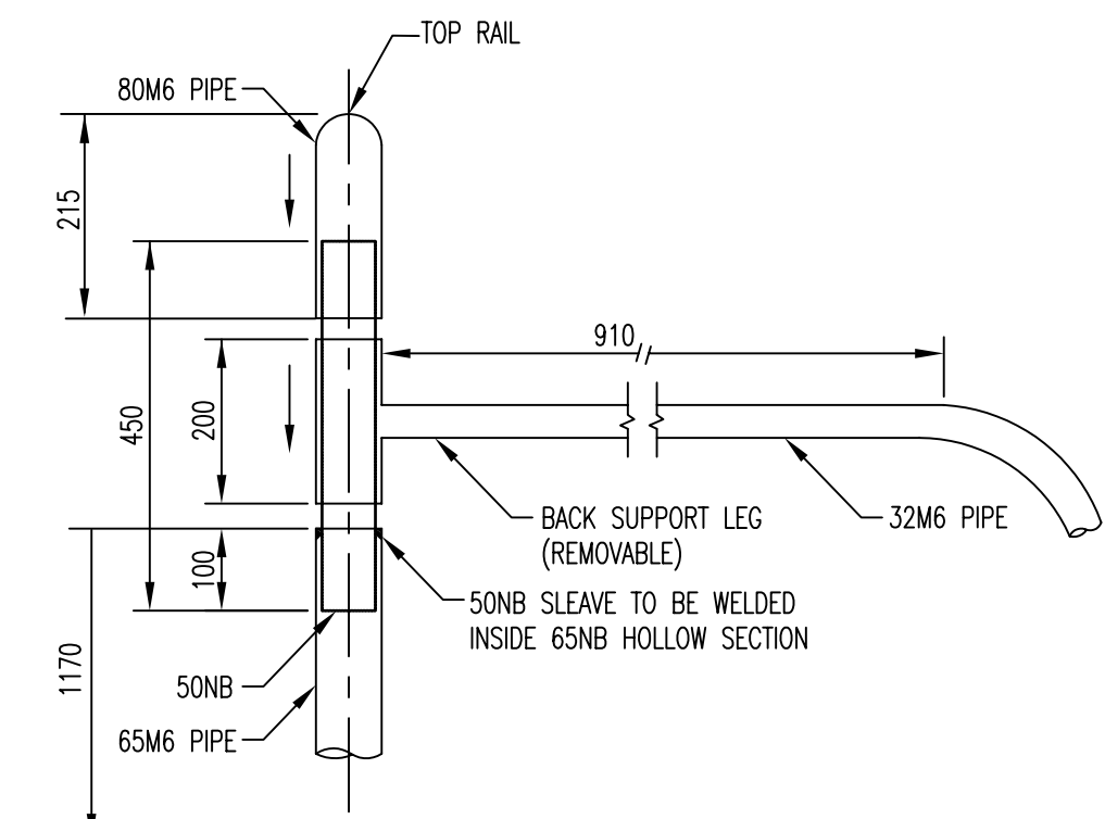
DETAIL 1 (NOT TO SCALE)
