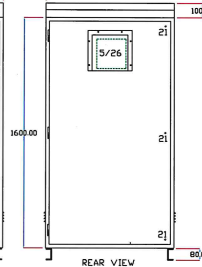
REAR VIEW
