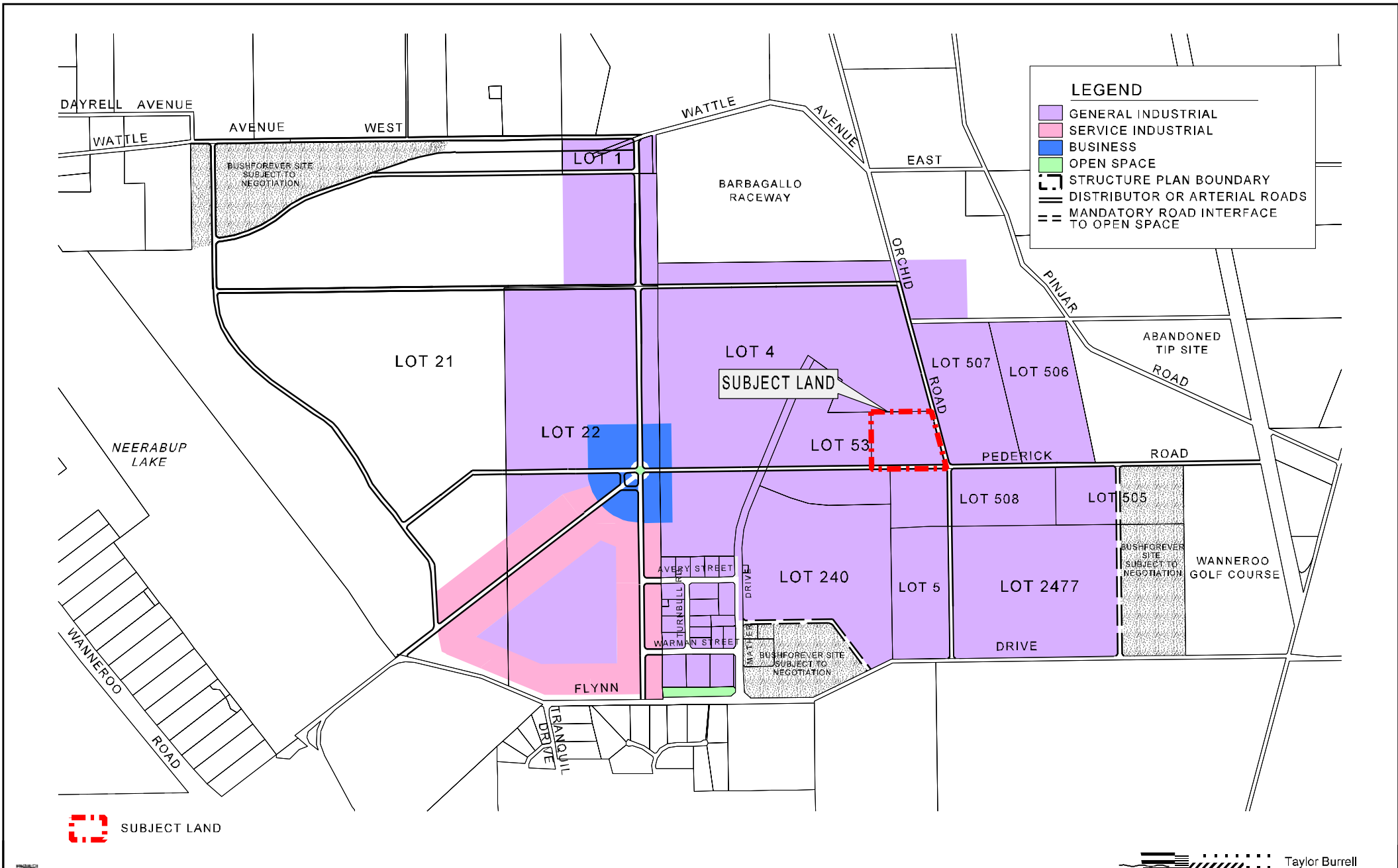
STRUCTURE PLAN CONTEXT DRAFT NEERABUP INDUSTRIAL AREA S.P. (No. 17)
