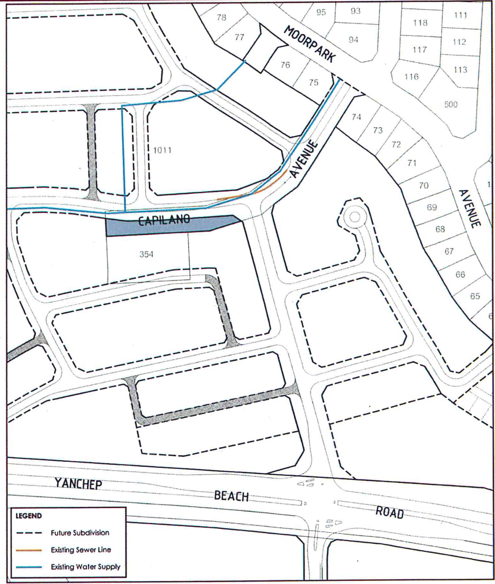
RE-ALIGNMENT OF CAPILANO AVENUE SCALE 1:2000
