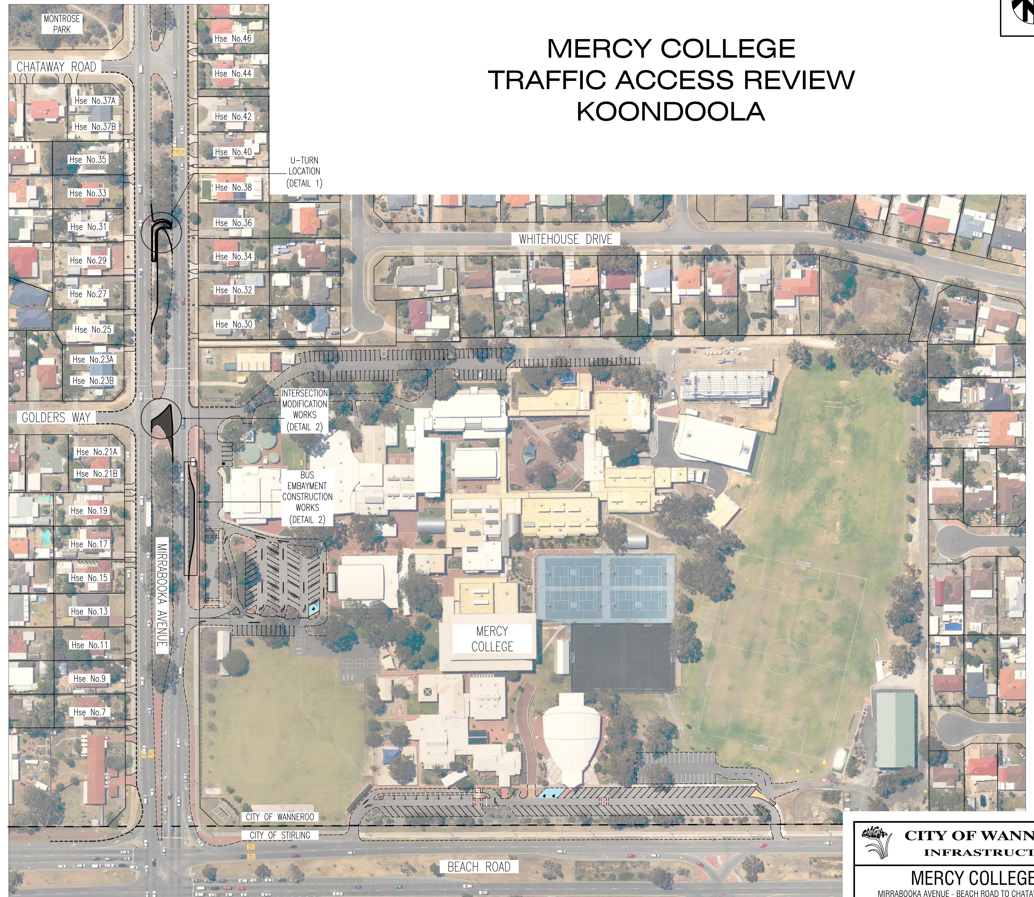
OVERVIEW PLAN (SCALE 1:1000)
