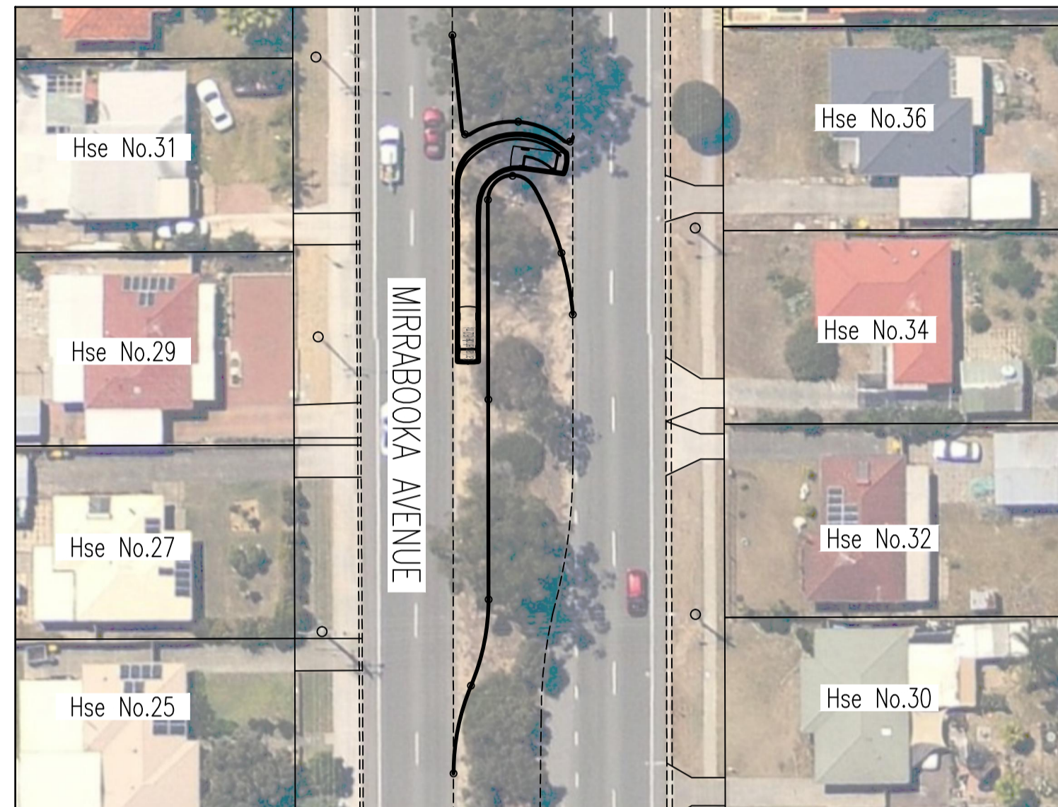
PROPOSED U-TURN DETAIL 1 (SCALE 1:500)
