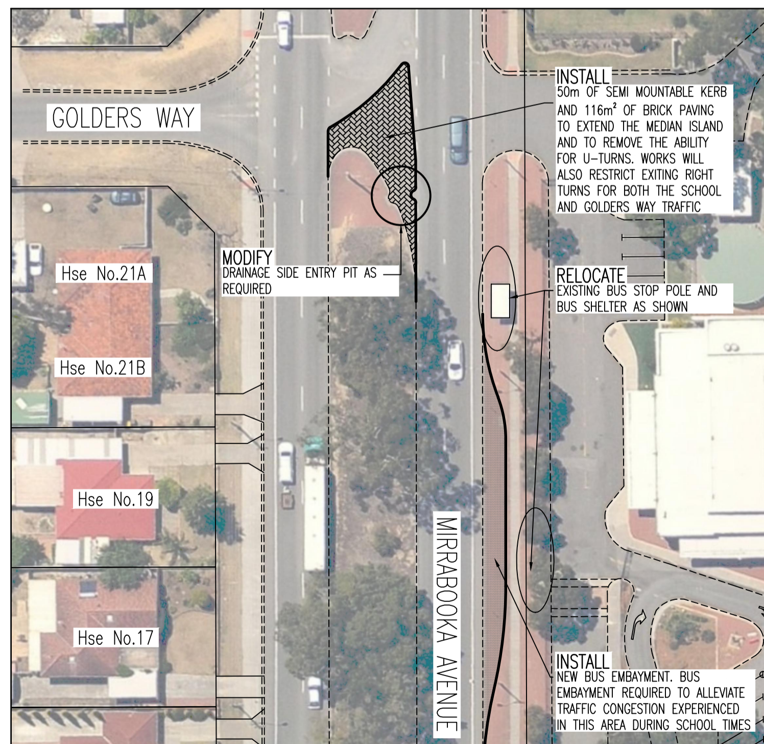
INTERSECTION MODIFICATION AND BUS EMBAYMENT WORKS DETAIL 3 (SCALE 1:500)
