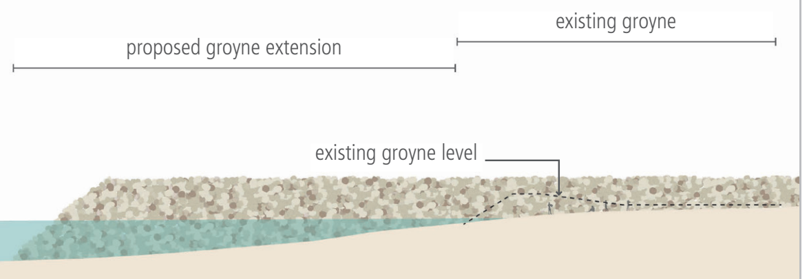
Location Plan - Section D
