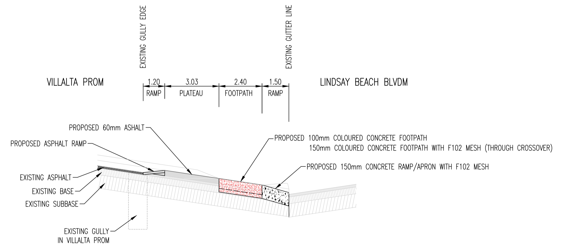
SECTION THROUGH MODIFIED ENTRY (LOOKING SOUTH) Scale Hor 1:100 Ver 1:25
