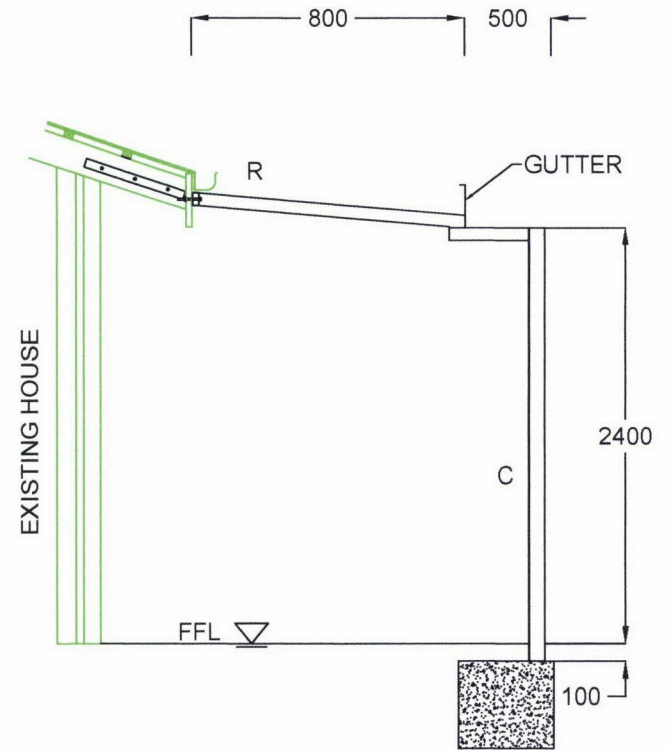
SECTION B FFL = HOUSE FFL
