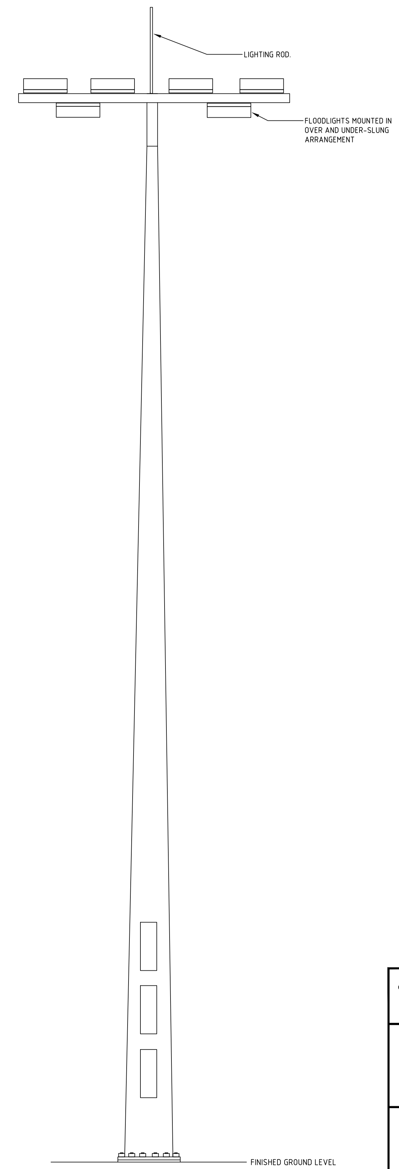
TYPICAL POLE ARRANGEMENT DETAIL NOT TO SCALE
