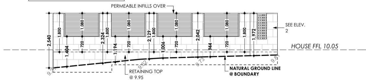
FRONT ELEVATION 1
