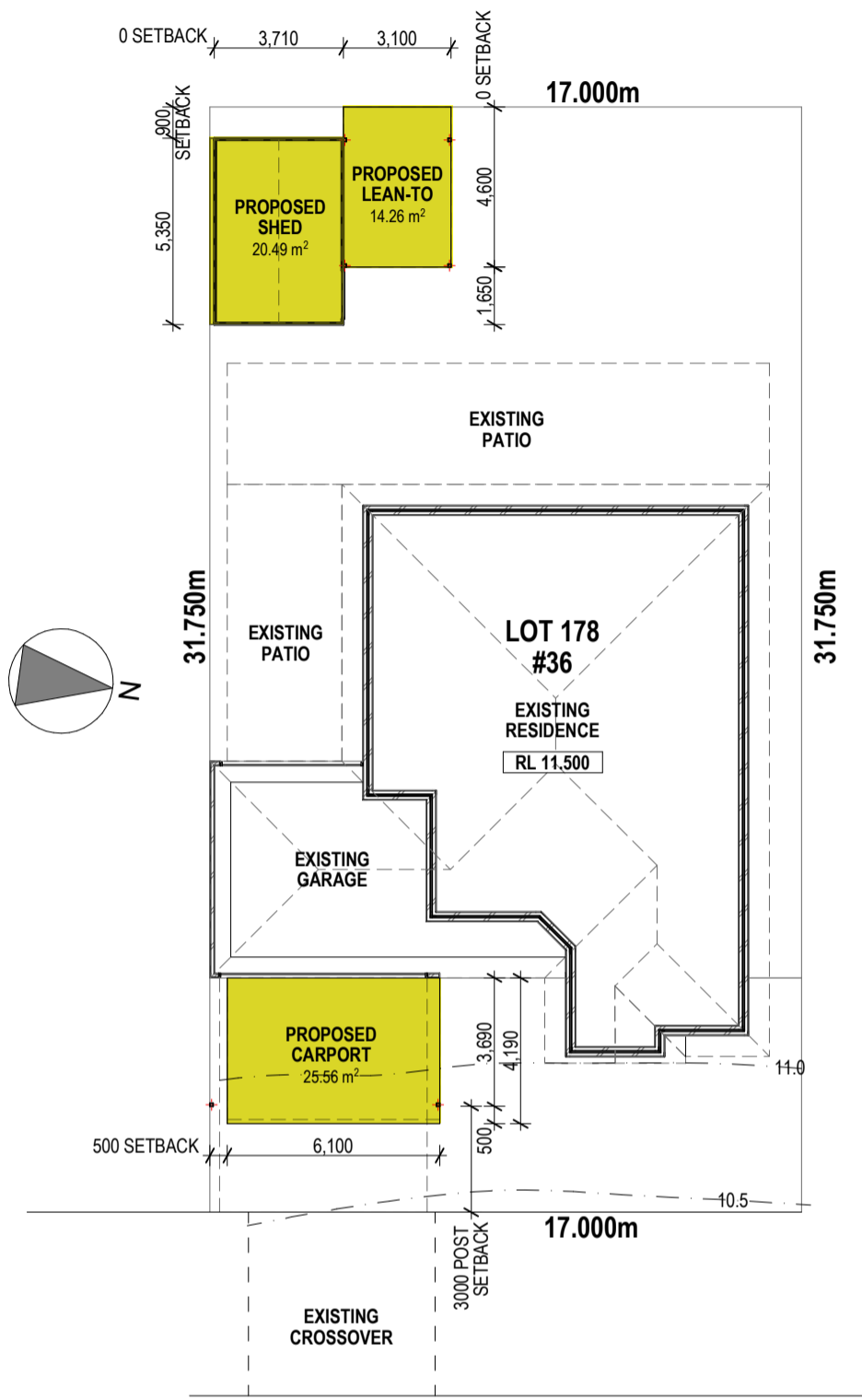
LITHGOW DRIVE SITE PLAN (1:200)
