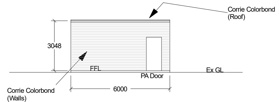
ELEVATION D
