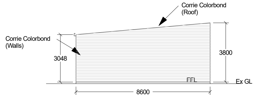
ELEVATION C
