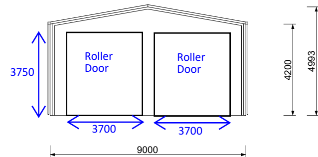
Garaport Wall with the Roller Doors
