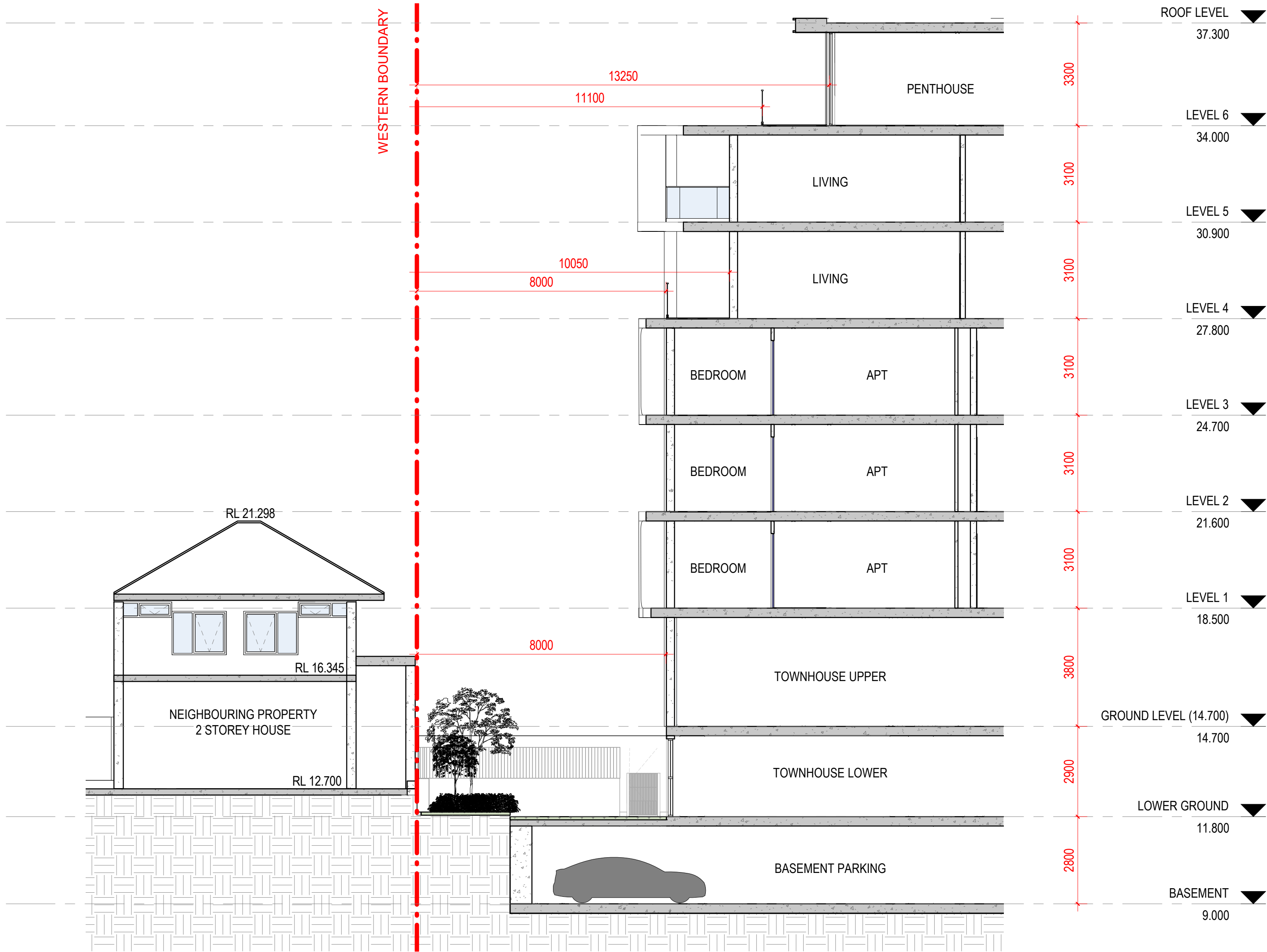
1 Section - Western Boundary A09-002 1 : 100
