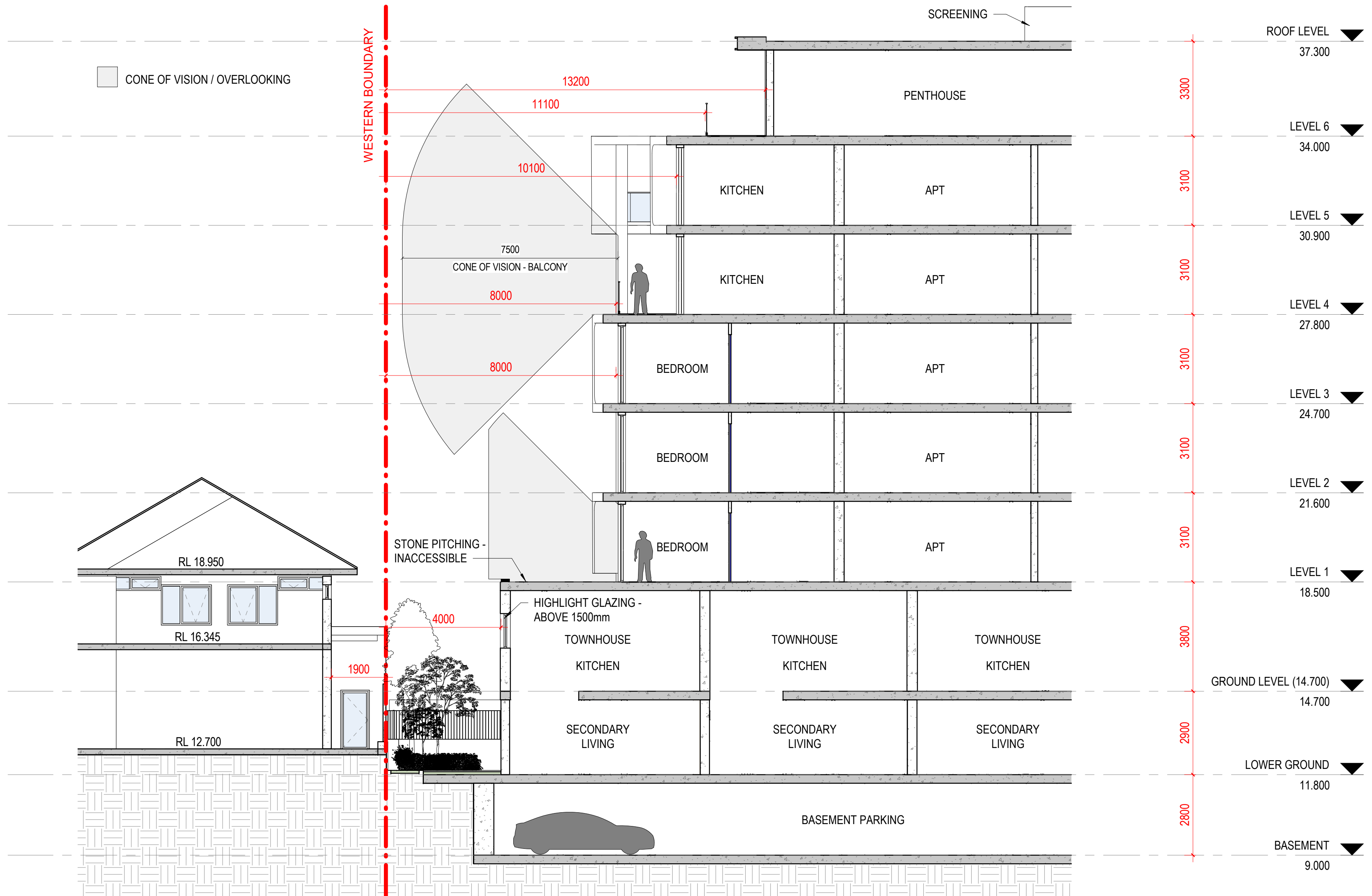
1 SECTION - WEST BOUNDARY_FRONT A09-002 1:100
