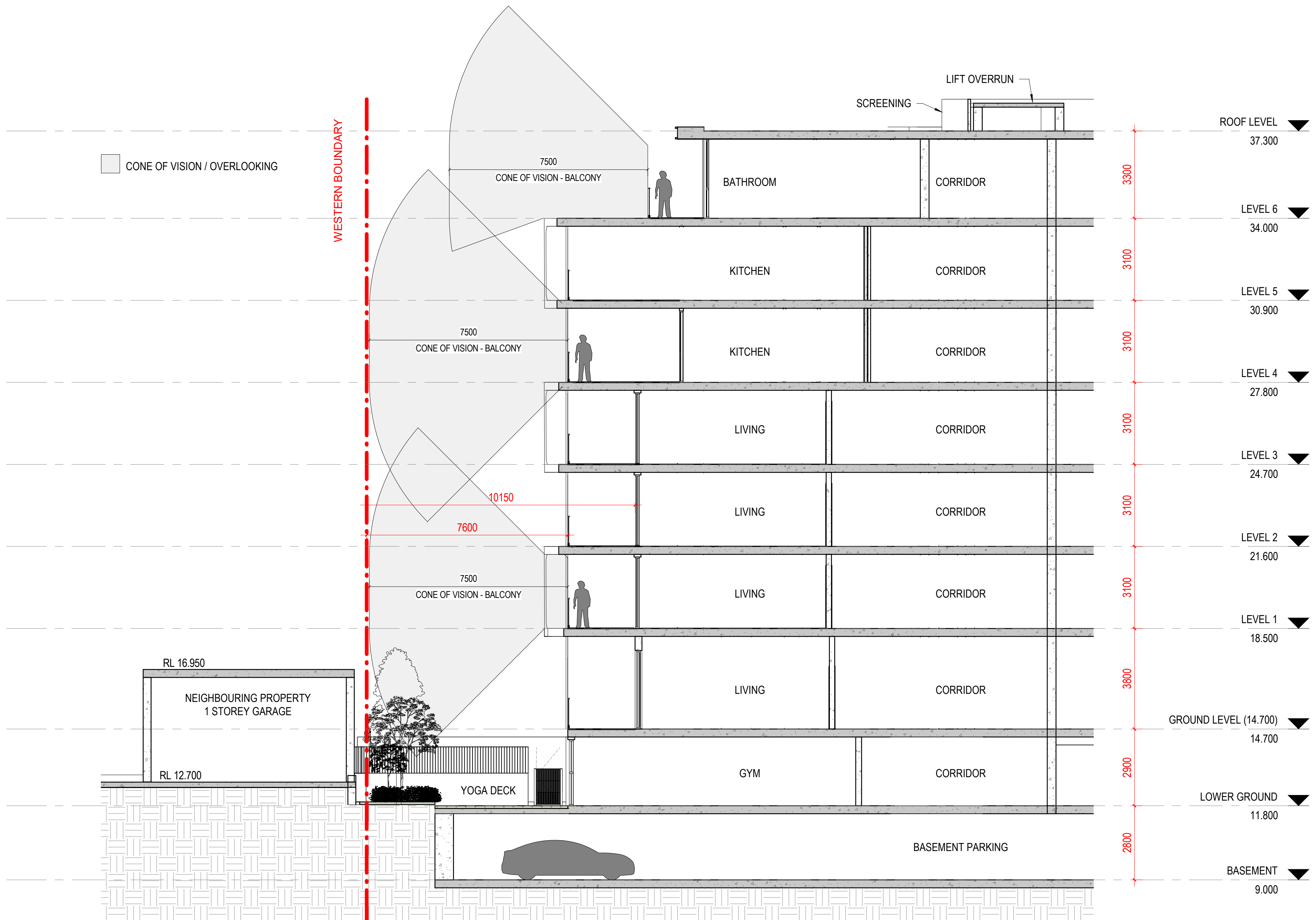
1 SECTION - WEST BOUNDARY A09-002 1 : 100
