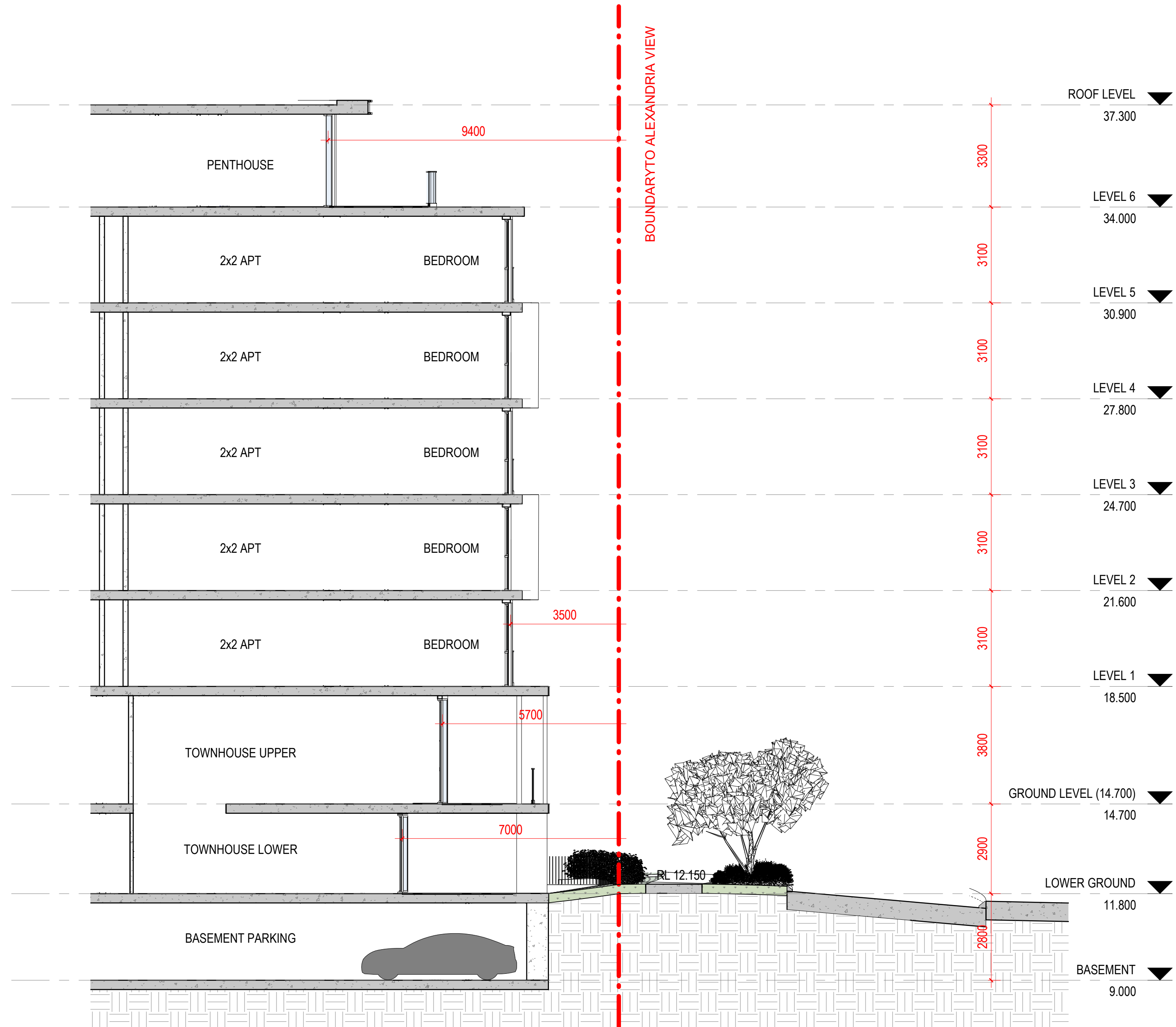
1 SECTION - ALEXANDRIA VIEW A09-002 1 : 100
