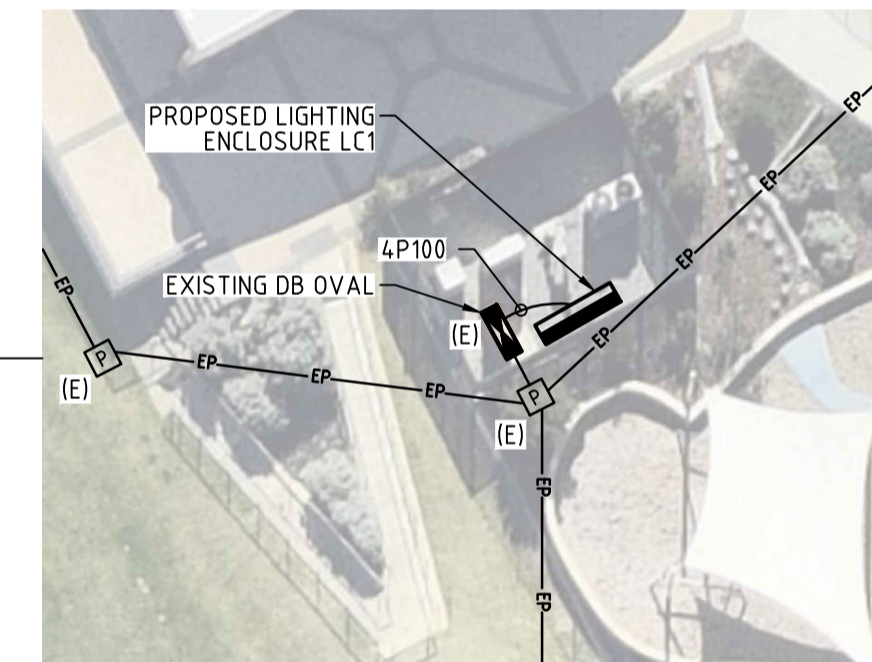
COMPOUND LAYOUT FOR CLARITY SCALE 1:250
