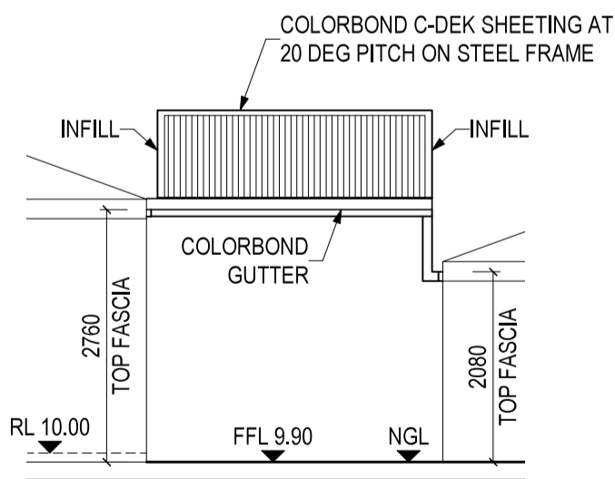
NORTH ELEVATION Scale: 1:75
