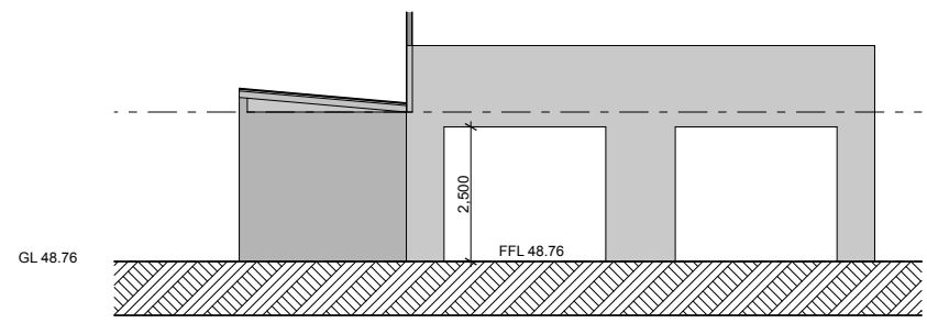
S-05 Section 1:100
