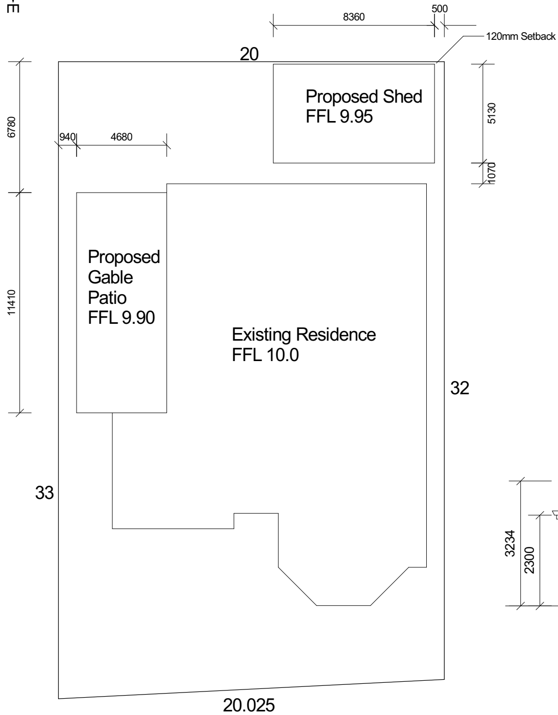
Brookway Retreat Scale 1:200
