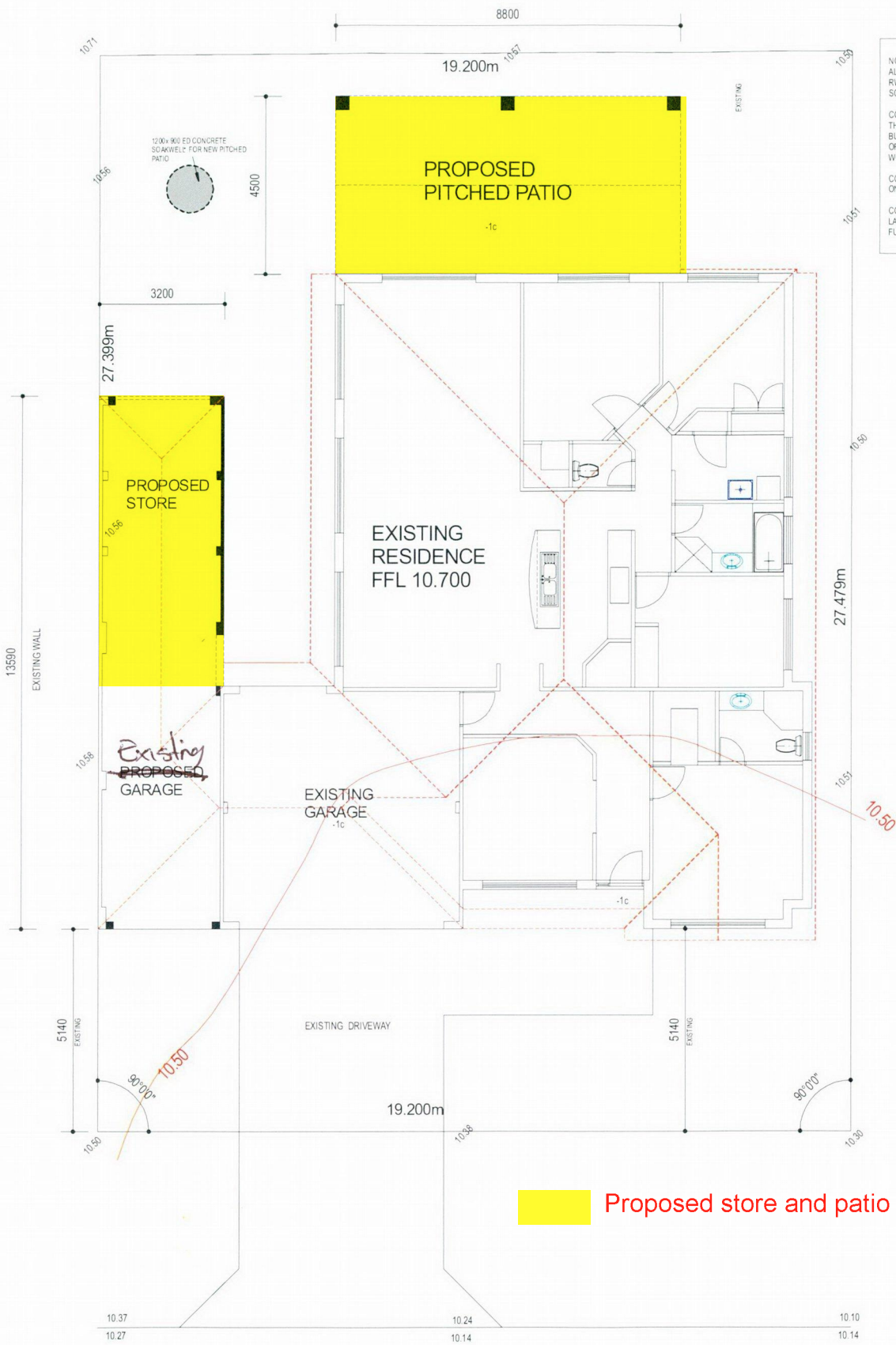
PROPOSED SITE PLAN 1:100
