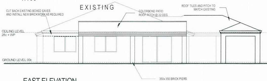
EAST ELEVATION 1:100
