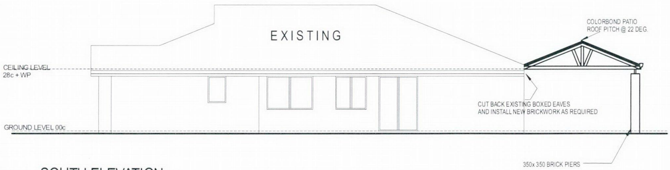
SOUTH ELEVATION 1:100
