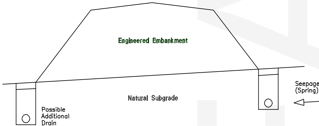
Figure D4.3 - Foundation Drains
