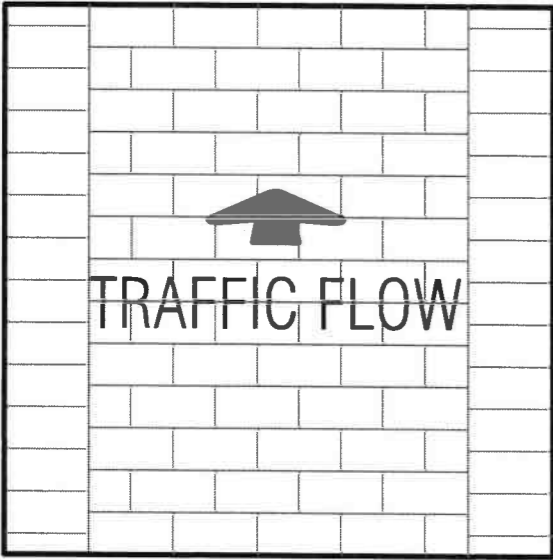
STRETCHER BOND (RECTANGULAR) (230 x 115mm STANDARD)
