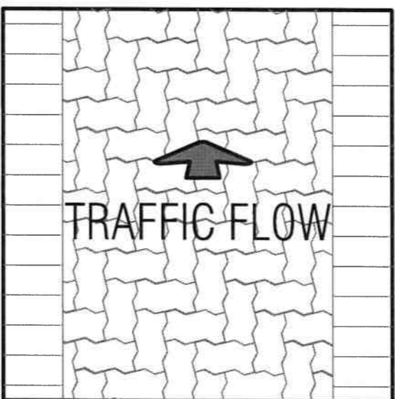
90 DEGREE HERRINGBONE (230 x 115mm INTERLOCK)
