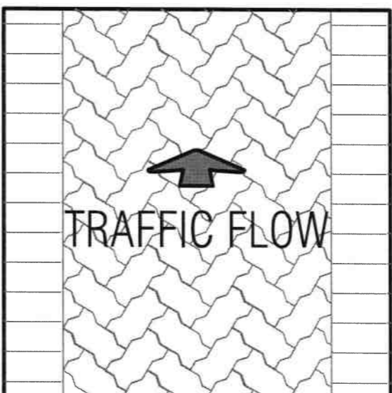
45 DEGREE HERRINGBONE (230 x 115mm INTERLOCK)
