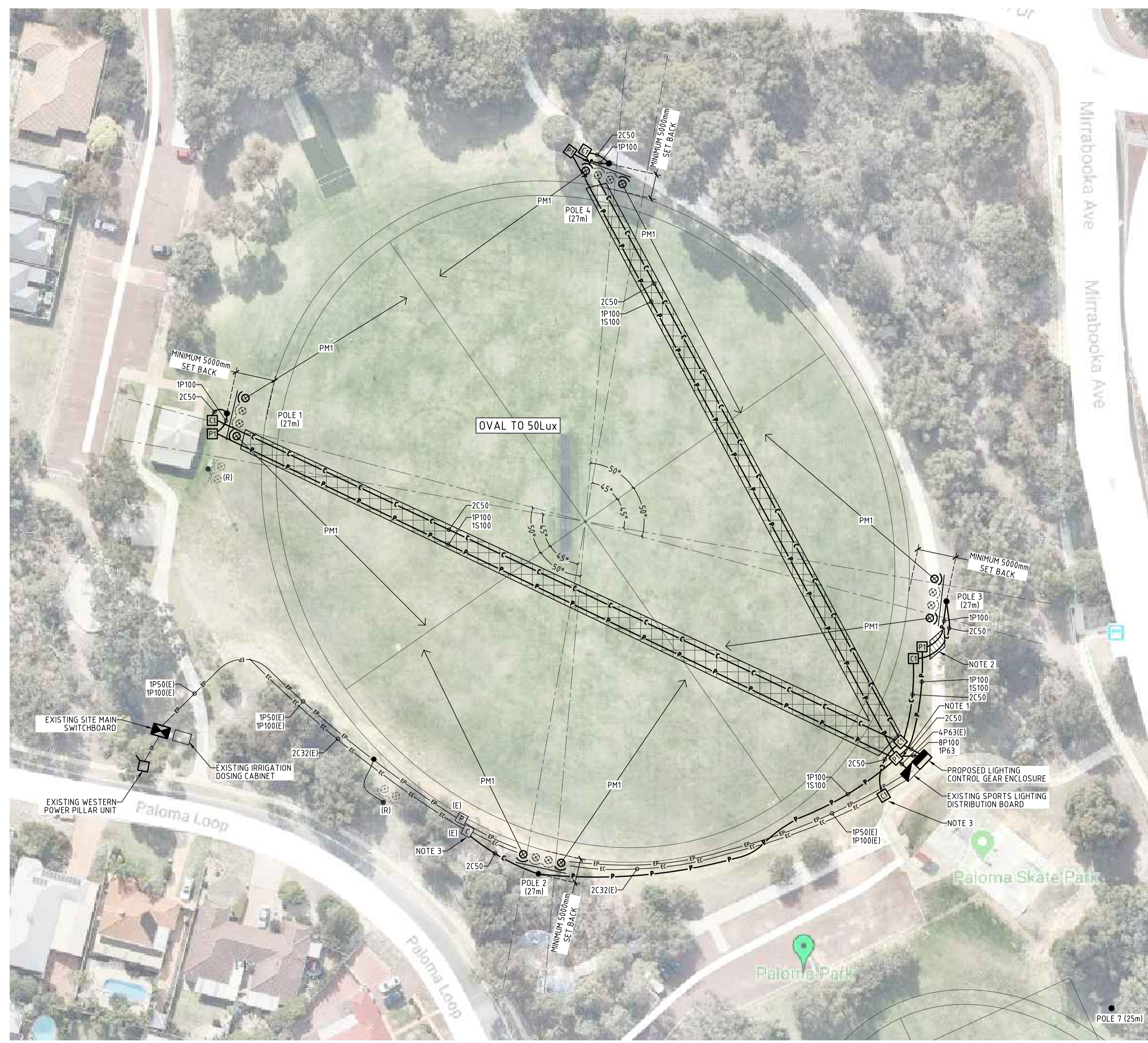
SITE PLAN - SPORTS LIGHTING LAYOUT SCALE 1500 @ A1
