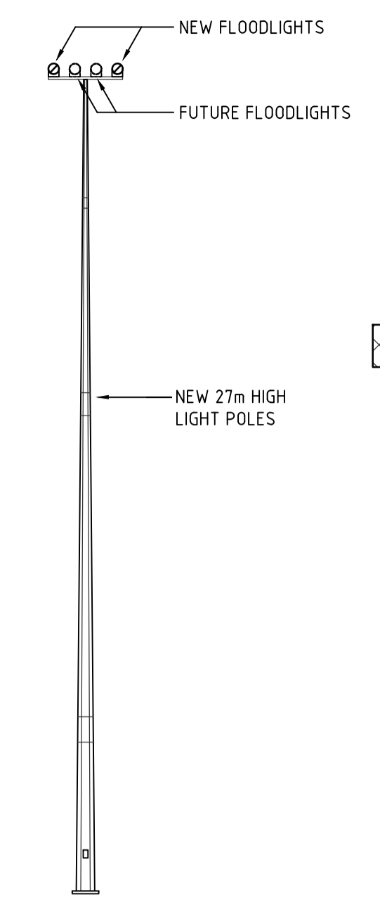
TYPICAL LIGHTING COLUMN DETAIL (POLES 1-4) SCALE N.T.S.
