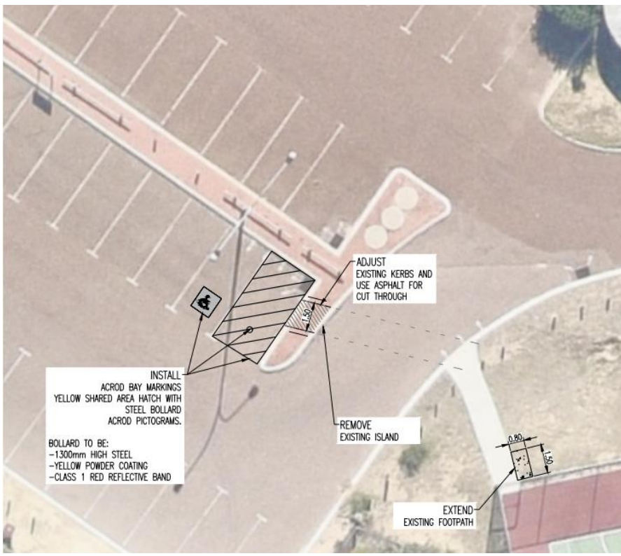
CONSTRUCTION PLAN REF: 3901-2-0
