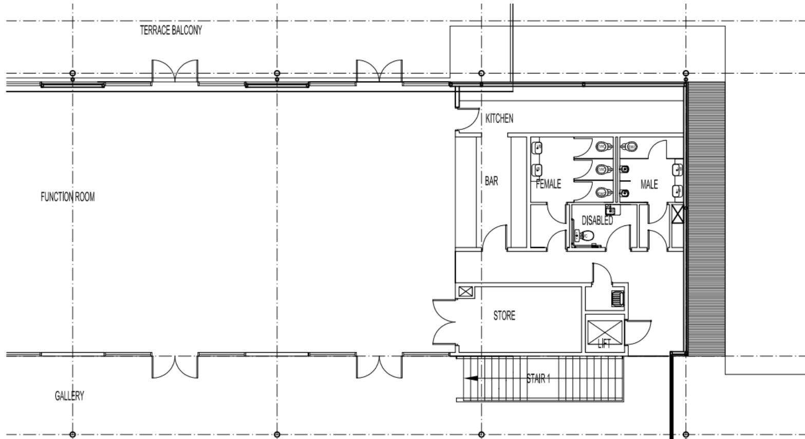
UPPER FLOOR NEW WORKS PLAN
