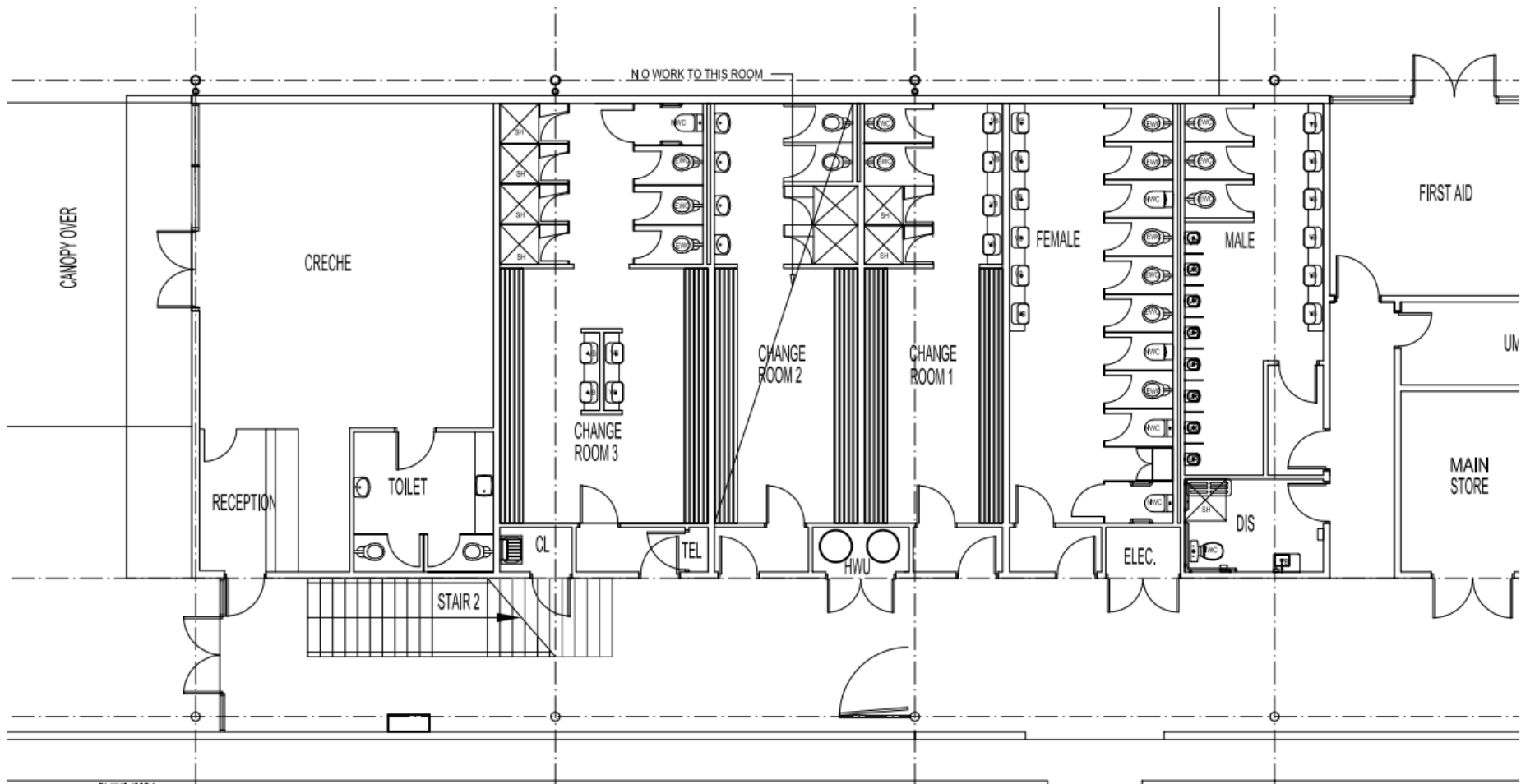
GROUND FLOOR NEW WORKS PLAN
