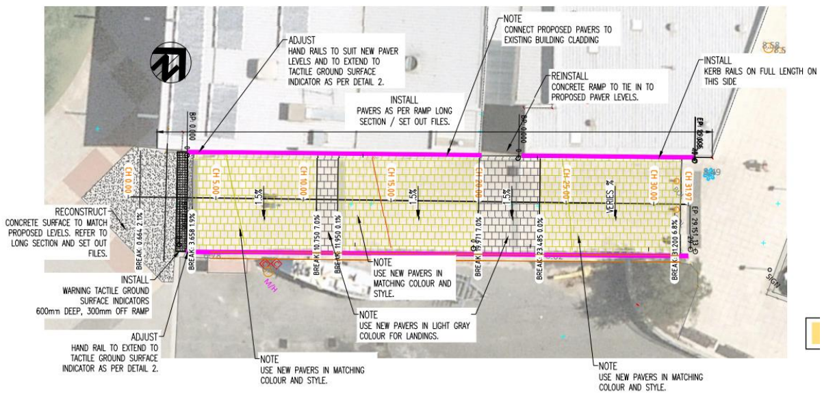
CONSTRUCTION PLAN REF: 3834-2-0
