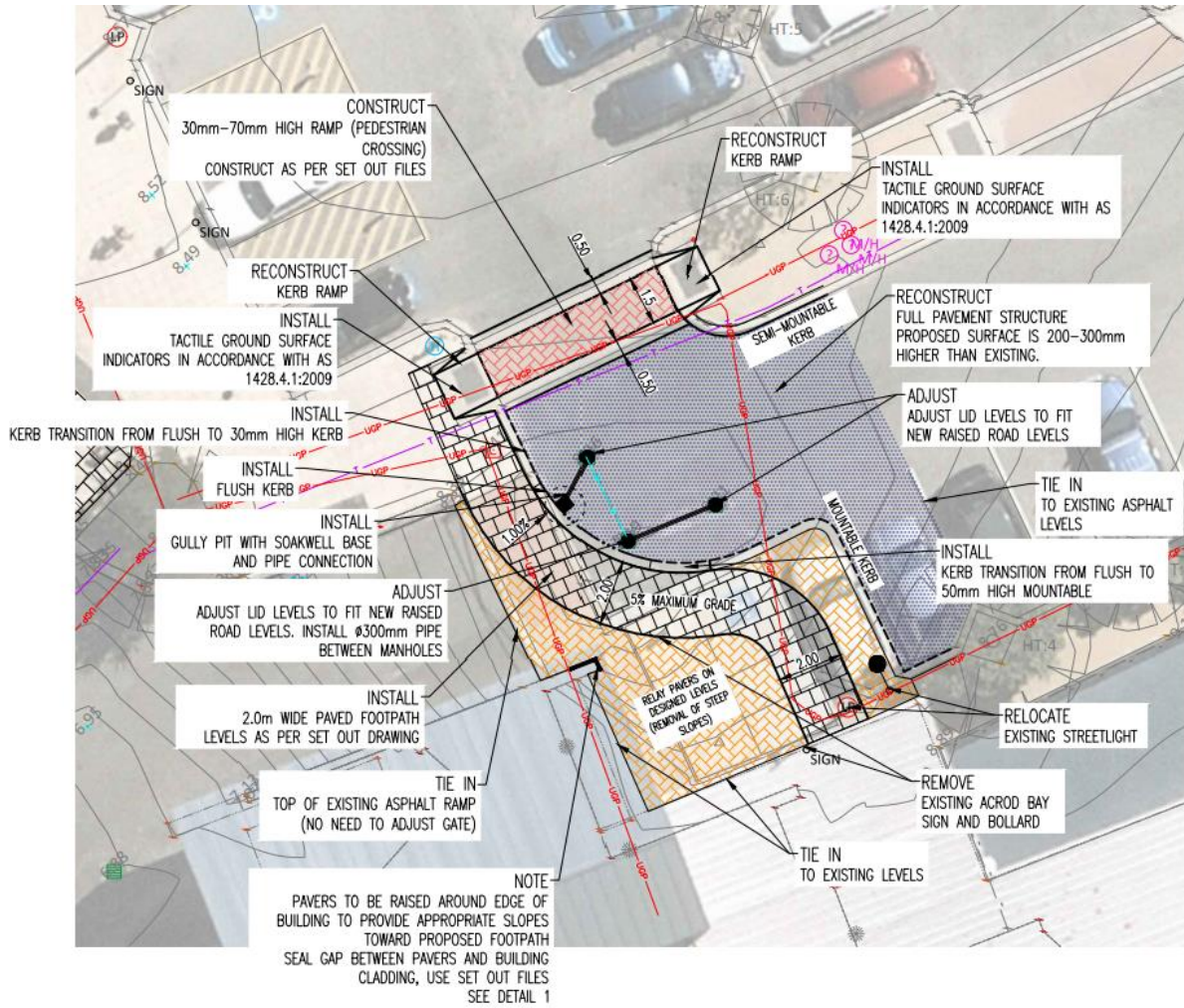
CONSTRUCTION PLAN REF: 3834-1-2
