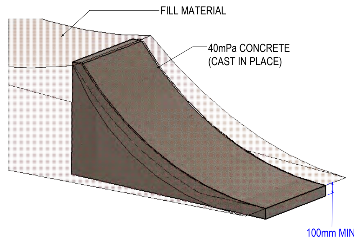
DETAIL A CONCRETE JUMP LIP- TYPICAL DETAIL
